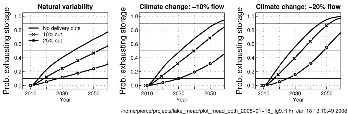
Figure 9. Effects of management strategies on likelihood of the Powell/Mead system dropping to deal pool elevations. Solid curve: when all requested water deliveries are supplied. Curves with crosses and circles: when deliveries are cut 10 and 25%, respectively, when total storage drops below 15 maf. Left panel: for current conditions. Middle and right panel: when runoff in the Colorado River system drops 10% and 20%, respectively, due to climate change.
