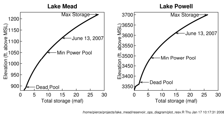
Figure 2. Total reservoir storage in Lakes Mead and Powell (million acre feet) as a function of lake surface elevation above mean sea level (ft). (We retain the units commonly used in the operation of these reservoirs; data are from CROSS [2007].) Arrows indicate the maximum storage possible in each Lake, the amount present on 13 June 2007, the minimum needed to enable hydroelectric power generation, and the minimum below which no more water can be extracted from the reservoir by gravity (“dead pool”). “Live storage” is all current storage above the dead pool elevation.
