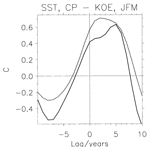
FIG. 22. Correlation between winter (JFM) time series in the central Pacific and KOE regions as a function of lag in years for observations (solid) and results from ECHO-2 (dotted connected by thin line). The ECHO-2 results were averaged over the regions CP and KOE shown in Fig. 9. Observations are based on COADS (Cayan 1992). Winter values were detrended and smoothed with a normalized 1–2–3–2–1 filter prior to calculation of the correlation. The central Pacific region is taken as an irregular shape between 30^{\circ}\text{N} – 45^{\circ}\text{N} and 180^{\circ} – 150^{\circ}\text{W} based on the leading North Pacific EOF. The KOE region covers 145^{\circ} – 170^{\circ}\text{E} , along 40^{\circ}\text{N} . Positive lags indicate that central Pacific time series leads.
