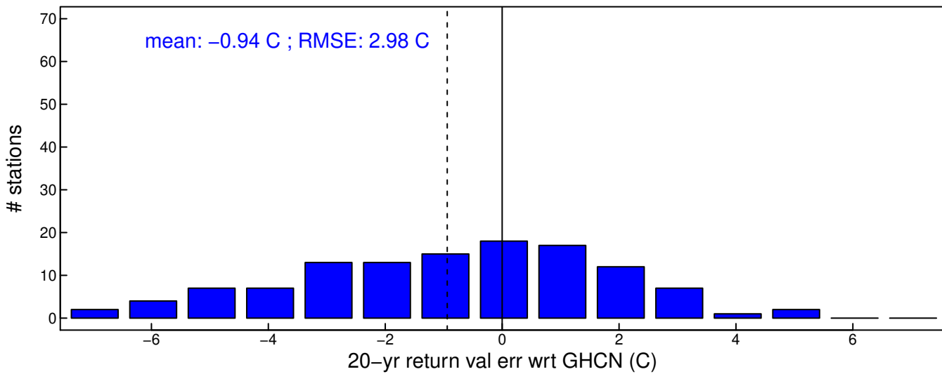
WRFBC err in 20-yr ret val wrt GHCN (C)
