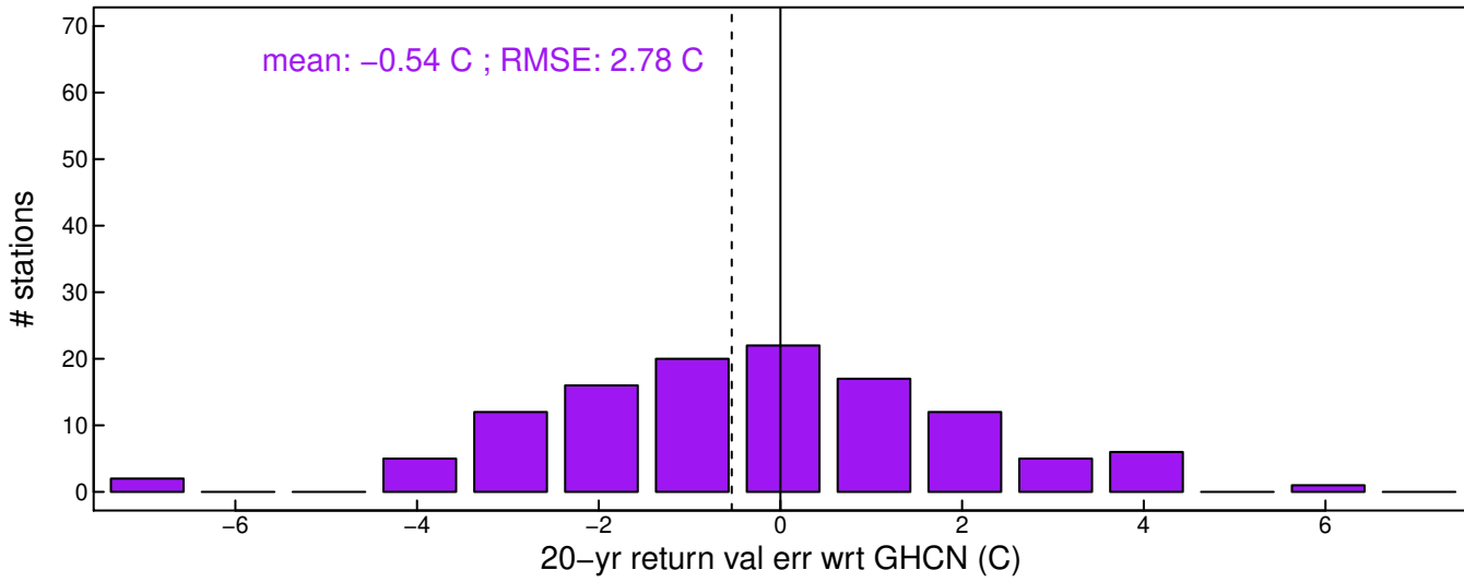
WRF err in 20-yr ret val wrt GHCN (C)
