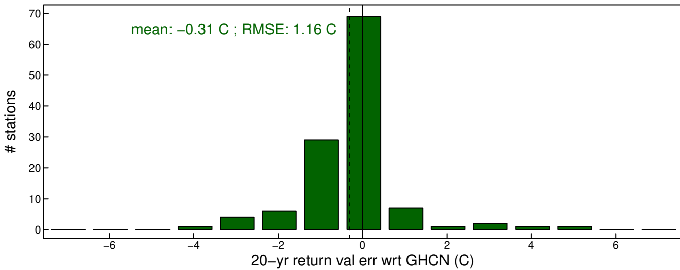
LIV err in 20-yr ret val wrt GHCN (C)
