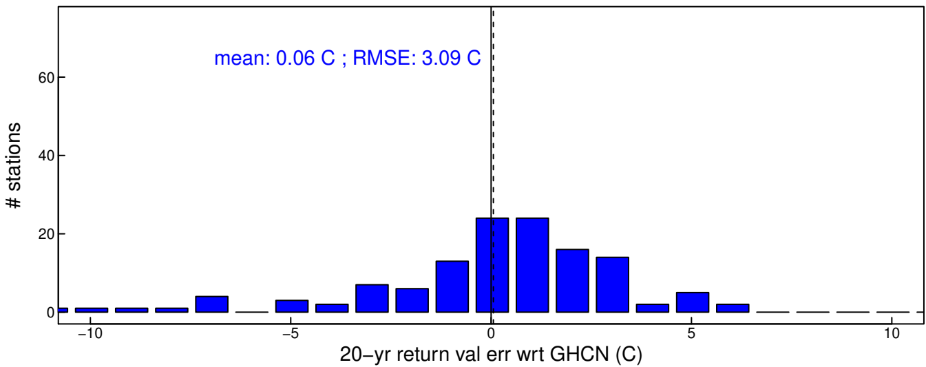
WRFBC err in 20-yr ret val wrt GHCN (C)
