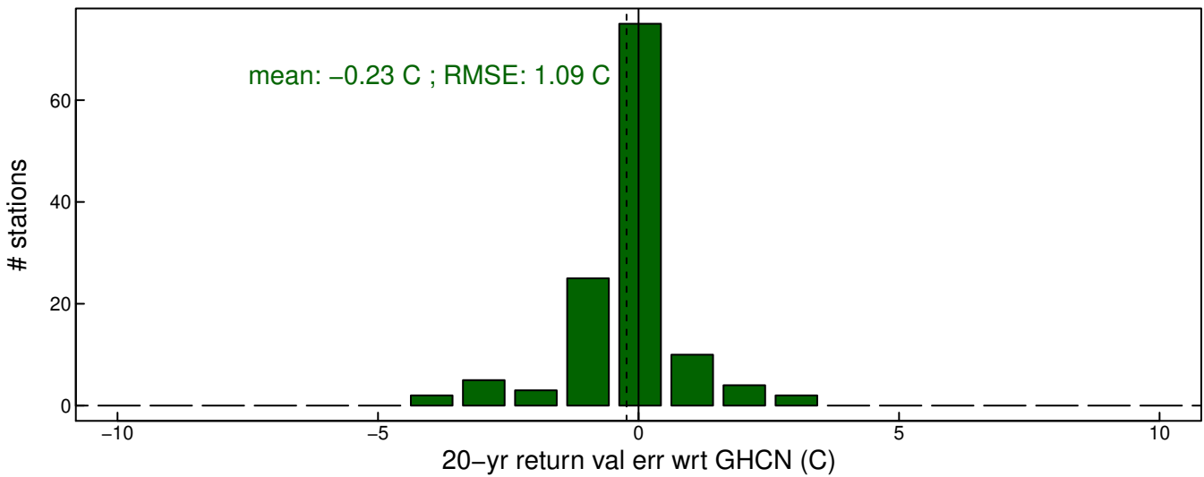
LIV err in 20-yr ret val wrt GHCN (C)
