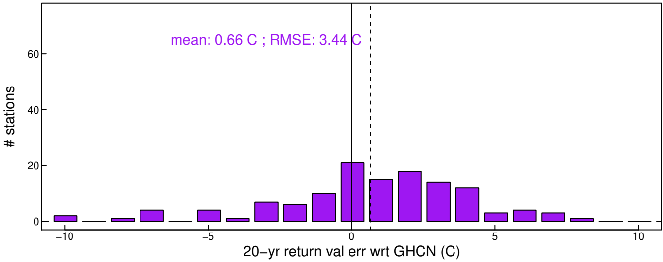
WRF err in 20-yr ret val wrt GHCN (C)
