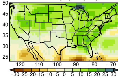
MRI-ESM2-0 pr yearly ssp370
