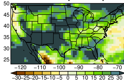
UKESM1-0-LL pr JJA ssp585
