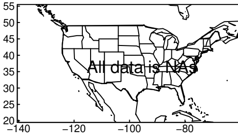
NorCPM1 pr JJA ssp370
