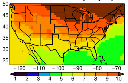
UKESM1-0-LL tasmax yearly ssp585
