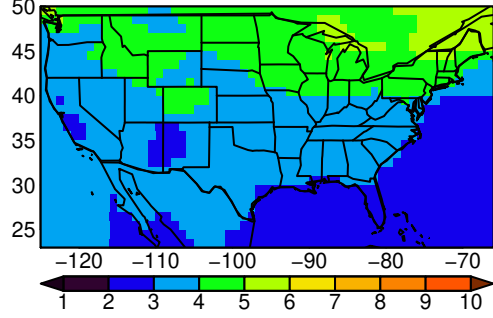
HadGEM3-GC31-LL tasmin JJA ssp2
