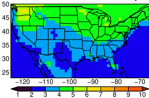
ACCESS-ESM1-5 tasmax SON ssp24
