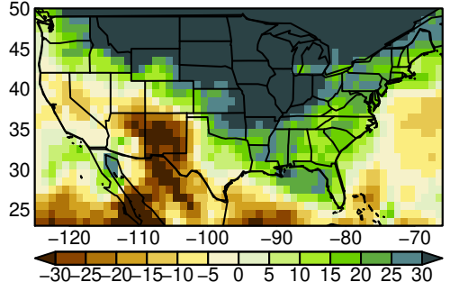
EC-Earth3 pr JJA ssp585
