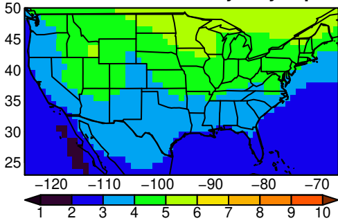
IPSL-CM6A-LR tasmin yearly ssp245
