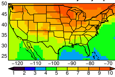
UKESM1-0-LL tasmax yearly ssp370
