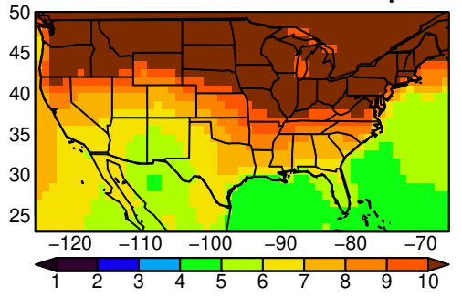
UKESM1-0-LL tasmax SON ssp585
