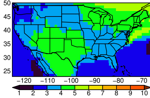
AWI-CM-1-1-MR tasmax JJA ssp37i
