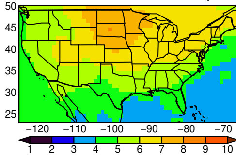
ACCESS-CM2 tasmax yearly ssp370
