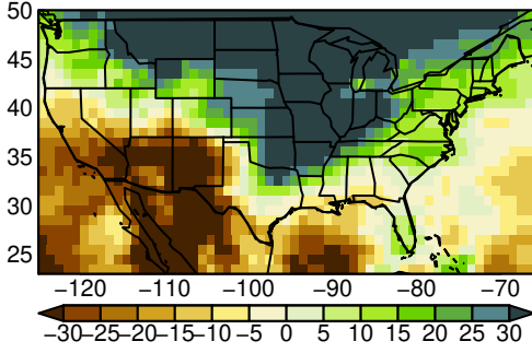
EC-Earth3 pr JJA ssp370
