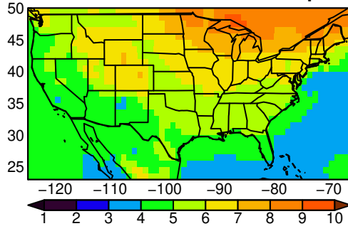
UKESM1-0-LL tasmin JJA ssp370
