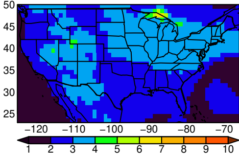
MRI-ESM2-0 tasmax JJA ssp245
