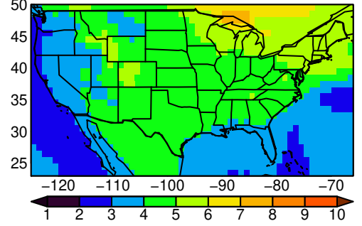
MRI-ESM2-0 tasmin JJA ssp585
