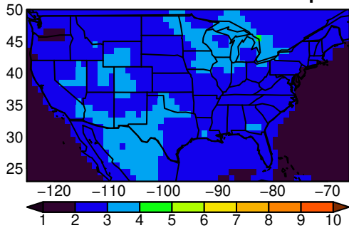
CNRM-ESM2-1 tasmin JJA ssp245
