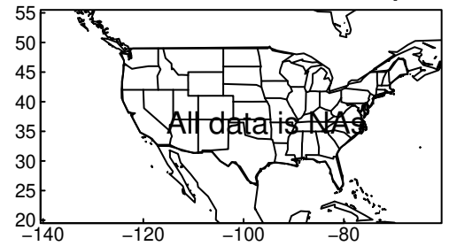
MPI-ESM1-2-LR tasmin JJA ssp585
