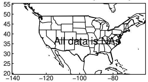
HadGEM3-GC31-MM pr JJA ssp585
