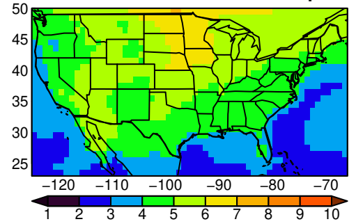
BCC-CSM2-MR tasmin yearly ssp585
