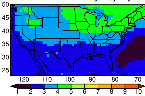
NorESM2-MM tasmx yearly ssp245
