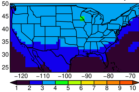
BCC-CSM2-MR tasmax yearly ssp245
