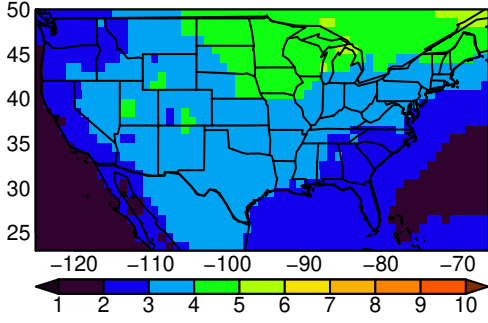
EC-Earth3-Veg tasmin JJA ssp245
