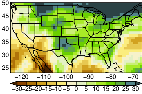
MRI-ESM2-0 pr JJA ssp245
