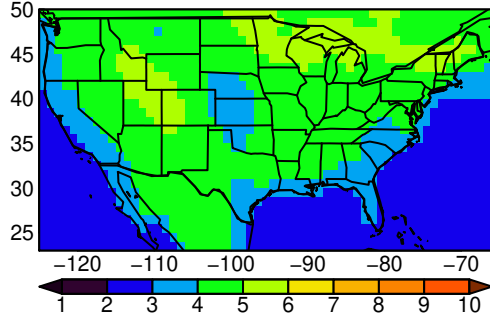
BCC-CSM2-MR tasmax JJA ssp370
