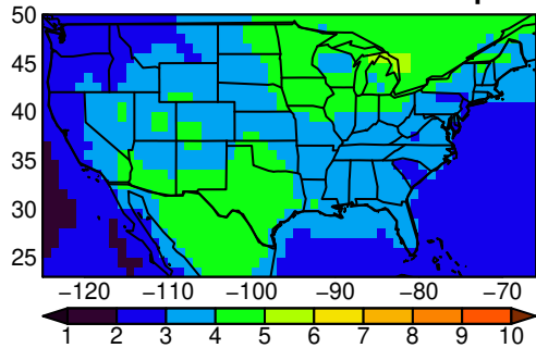
CNRM-ESM2-1 tasmin JJA ssp370
