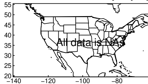
HadGEM3-GC31-MM tasmin yearly ssp5
