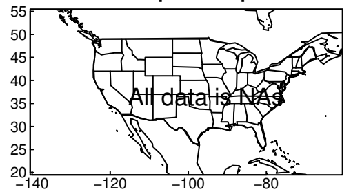
NESM3 pr JJA ssp585
