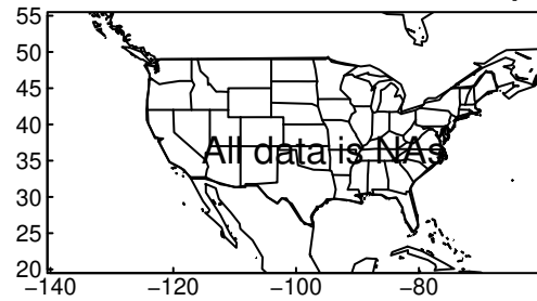
HadGEM3-GC31-MM tasmax JJA ssp2
