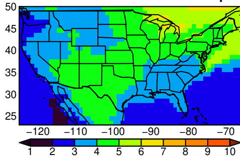
AWI-CM-1-1-MR tasmin JJA ssp37f
