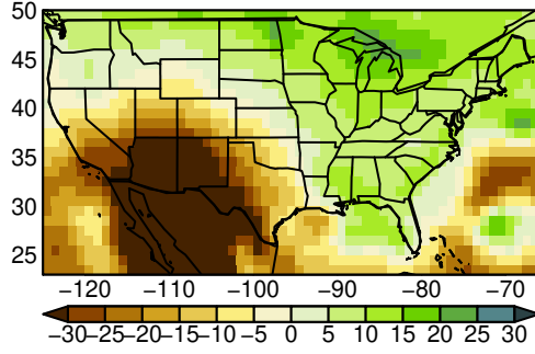
MPI-ESM1-2-LR pr JJA ssp370
