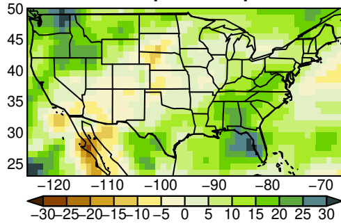
CESM2 pr yearly ssp370
