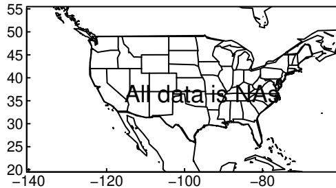
FGOALS-g3 pr yearly ssp585
