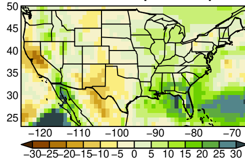
MPI-ESM1-2-HR pr yearly ssp370
