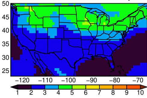
NorESM2-MM tasmx JJA ssp245
