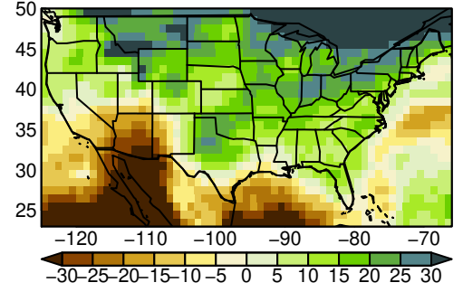
MRI-ESM2-0 pr JJA ssp585
