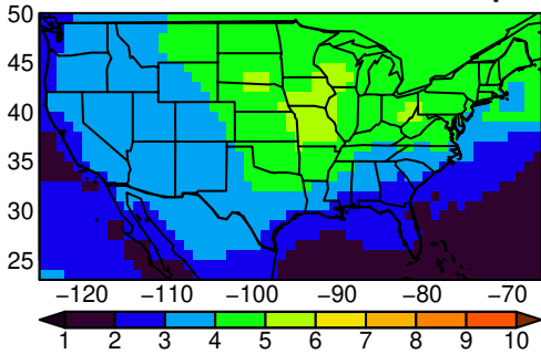
AWI-CM-1-1-MR tasmax yearly ssp24i
