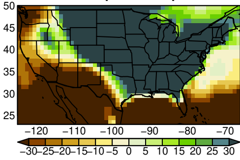
NESM3 pr JJA ssp245
