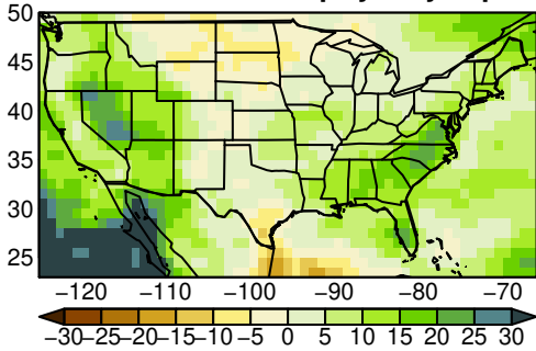
HadGEM3-GC31-LL pr yearly ssp245
