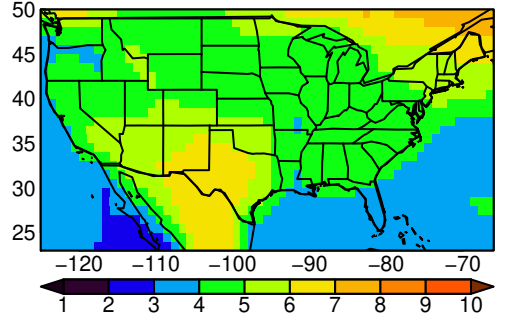
NESM3 tasmin JJA ssp585
