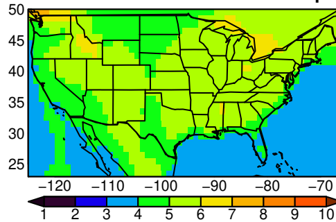
ACCESS-ESM1-5 tasmax JJA ssp58
