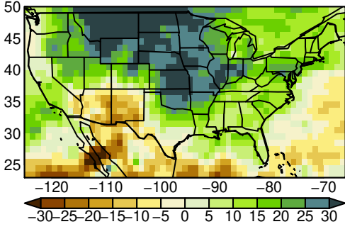
EC-Earth3 pr JJA ssp245
