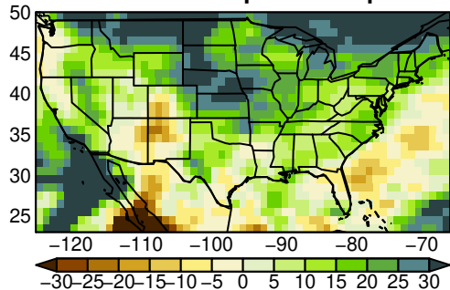
UKESM1-0-LL pr JJA ssp370
