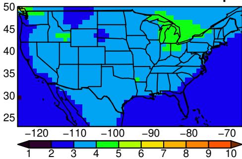
ACCESS-ESM1-5 tasmax JJA ssp24
