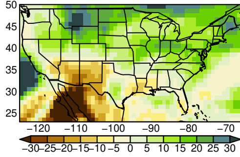
BCC-CSM2-MR pr JJA ssp370
