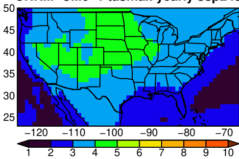
CNRM-CM6-1 tasmx yearly ssp245
