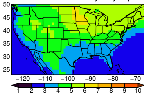
NorESM2-MM tasmx yearly ssp370
