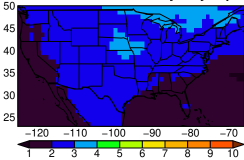
MPI-ESM1-2-HR tasmax yearly ssp24i
