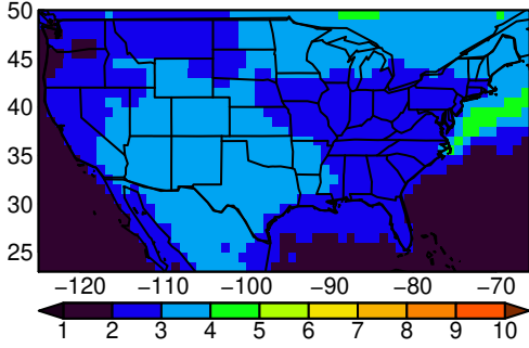
AWI-CM-1-1-MR tasmax JJA ssp24i
