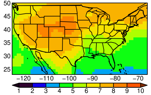
NESM3 tasmin yearly ssp585
