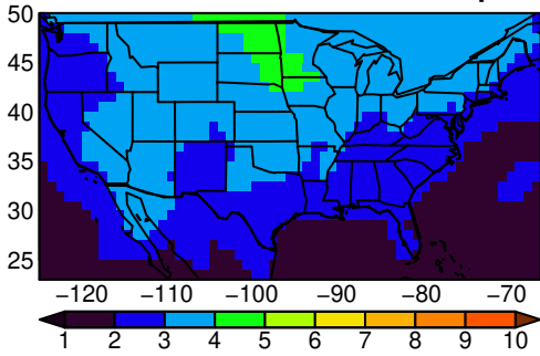
BCC-CSM2-MR tasmin yearly ssp245
