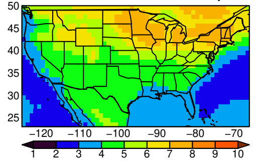
NorESM2-MM tasmx JJA ssp585
