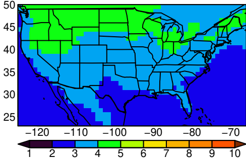
ACCESS-ESM1-5 tasmin SON ssp24i
