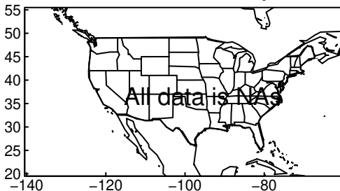
NESM3 tasmax DJF ssp370
