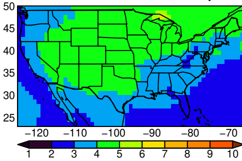
MRI-ESM2-0 tasmax yearly ssp370
