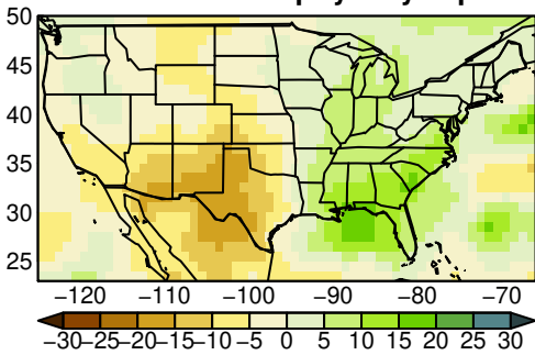
MPI-ESM1-2-LR pr yearly ssp245
