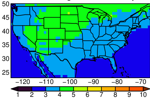
EC-Earth3-Veg tasmin yearly ssp245
