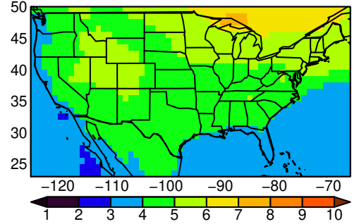
MRI-ESM2-0 tasmin yearly ssp585
