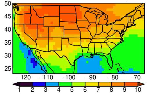
IPSL-CM6A-LR tasmin SON ssp585
