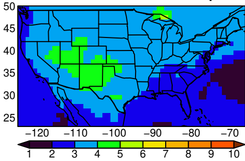
MRI-ESM2-0 tasmax yearly ssp245
