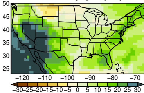
UKESM1-0-LL pr yearly ssp245
