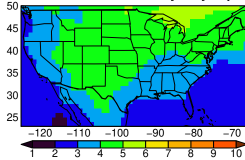
MPI-ESM1-2-LR tasmin yearly ssp370
