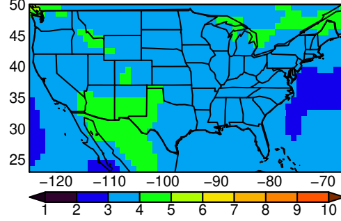
ACCESS-ESM1-5 tasmin JJA ssp37i
