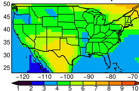
NESM3 tasmax JJA ssp585
