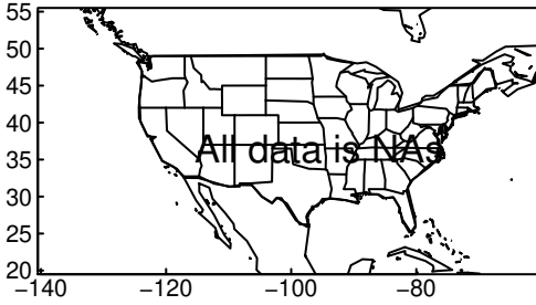
CNRM-CM6-1-HR tasmax JJA ssp37
