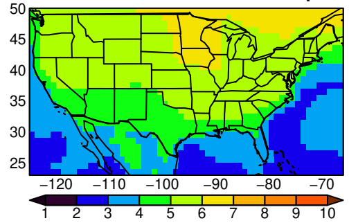
BCC-CSM2-MR tasmax yearly ssp585
