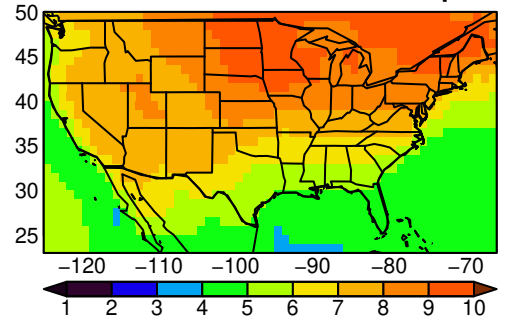
IPSL-CM6A-LR tasmax yearly ssp585
