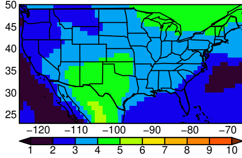
MPI-ESM1-2-LR tasmax JJA ssp37f
