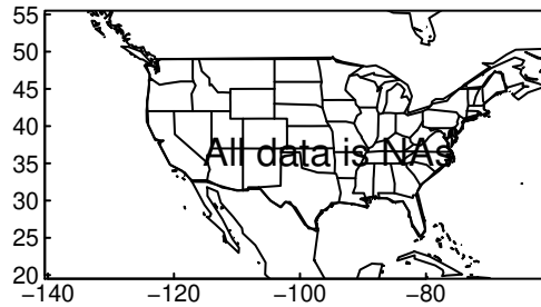
HadGEM3-GC31-LL tasmax yearly ssp3
