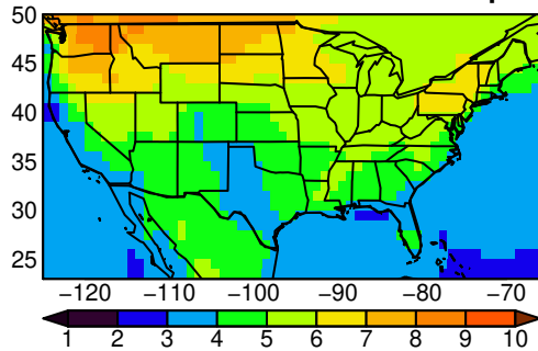
ACCESS-ESM1-5 tasmax SON ssp37
