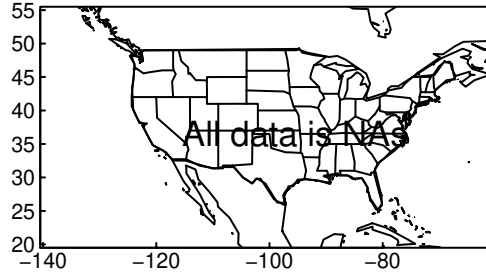
HadGEM3-GC31-LL tasmax DJF ssp3
