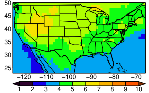
MRI-ESM2-0 tasmin SON ssp585
