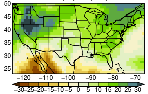
CESM2 pr yearly ssp585
