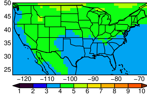
ACCESS-ESM1-5 tasmin yearly ssp37i
