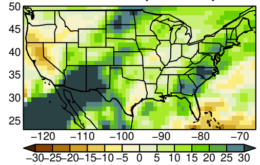
BCC-CSM2-MR pr yearly ssp585
