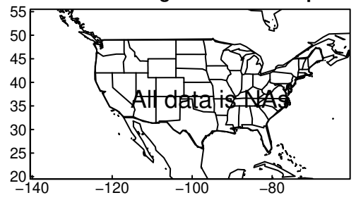
EC-Earth3-Veg tasmax JJA ssp585
