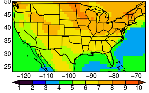
HadGEM3-GC31-LL tasmax JJA ssp5
