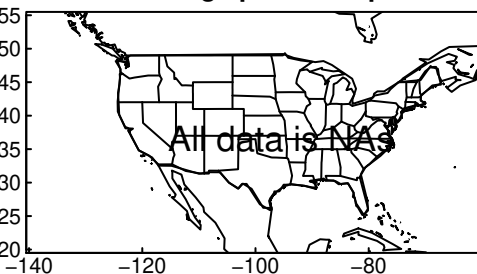
FGOALS-g3 pr SON ssp370
