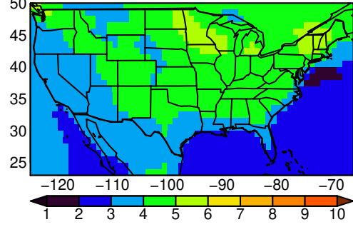
HadGEM3-GC31-LL tasmax JJA ssp2
