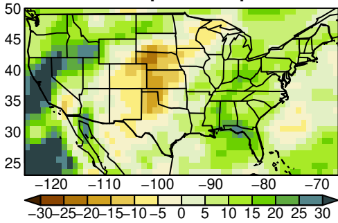
CESM2 pr yearly ssp245
