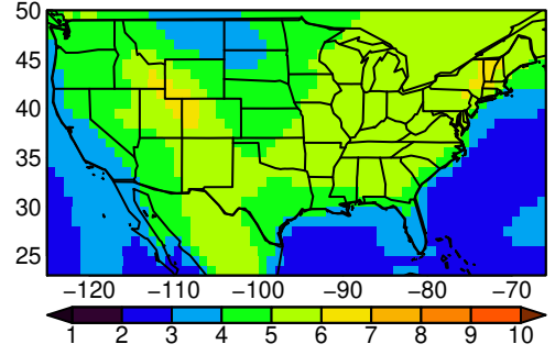
BCC-CSM2-MR tasmax JJA ssp585
