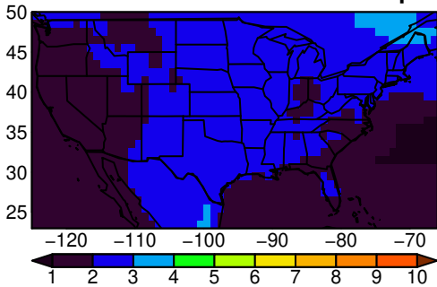
MPI-ESM1-2-HR tasmax JJA ssp24i
