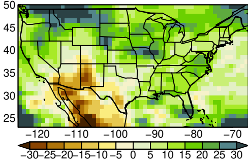
HadGEM3-GC31-LL pr JJA ssp245
