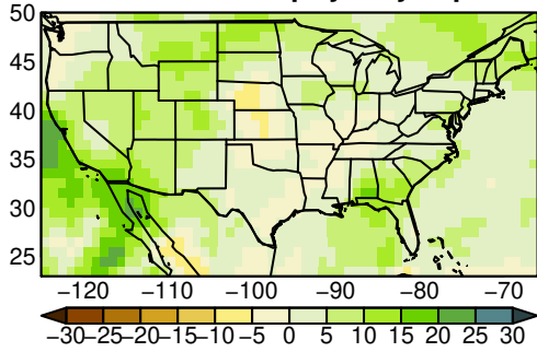
BCC-CSM2-MR pr yearly ssp245
