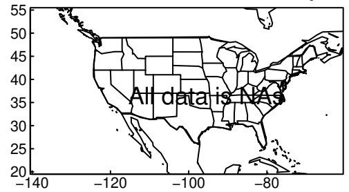
AWI-CM-1-1-MR tasmax JJA ssp58i
