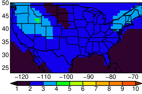
BCC-CSM2-MR tasmax JJA ssp245
