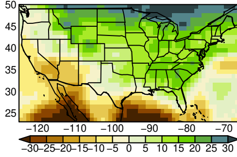
MRI-ESM2-0 pr JJA ssp370
