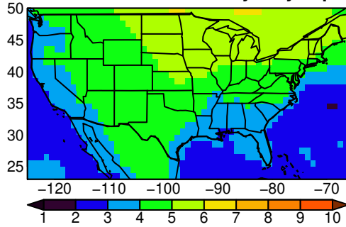
MPI-ESM1-2-HR tasmax yearly ssp58i
