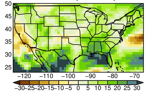
MRI-ESM2-0 pr yearly ssp585
