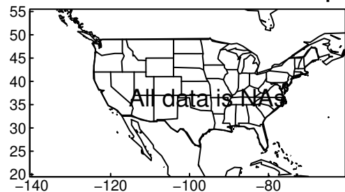
HadGEM3-GC31-MM tasmin JJA ssp2
