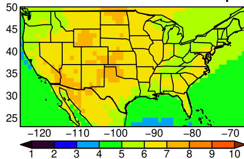
CNRM-CM6-1-HR tasmin yearly ssp5
