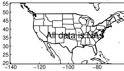
GISS-E2-1-G tasmin JJA ssp370
