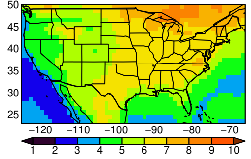
IPSL-CM6A-LR tasmin JJA ssp585
