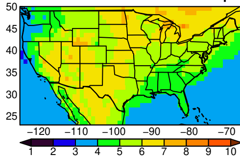
CNRM-CM6-1-HR tasmin JJA ssp58
