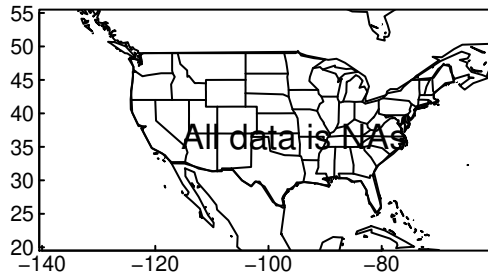
HadGEM3-GC31-LL tasmin yearly ssp3
