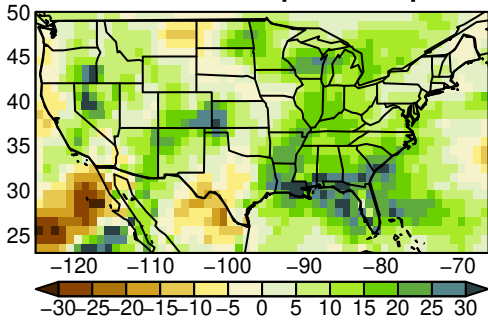
MPI-ESM1-2-HR pr yearly ssp245
