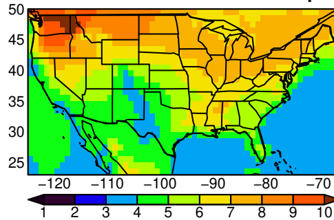
ACCESS-ESM1-5 tasmax SON ssp58
