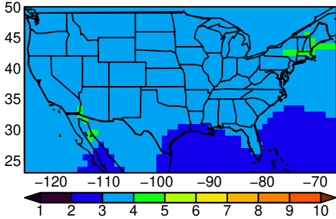
ACCESS-ESM1-5 tasmin yearly ssp24i
