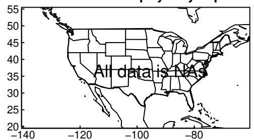
MPI-ESM1-2-LR pr yearly ssp585
