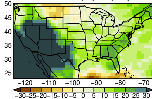
UKESM1-0-LL pr yearly ssp585
