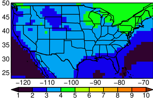
IPSL-CM6A-LR tasmax JJA ssp245
