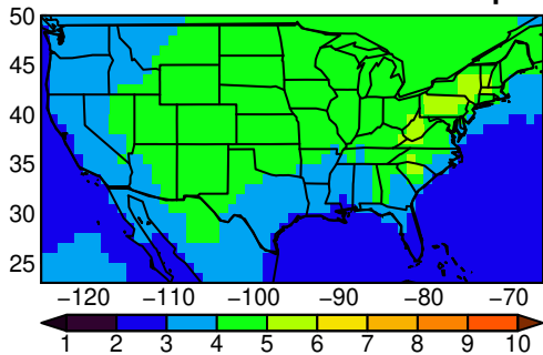
MPI-ESM1-2-HR tasmax yearly ssp37i
