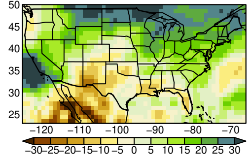
BCC-CSM2-MR pr JJA ssp585
