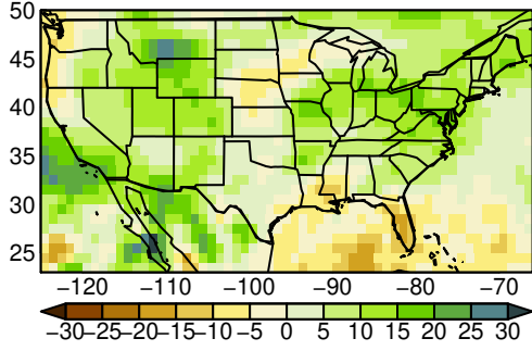
BCC-CSM2-MR pr JJA ssp245
