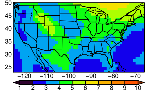
BCC-CSM2-MR tasmin JJA ssp585
