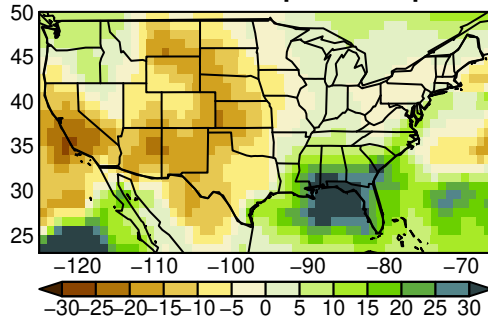
MPI-ESM1-2-LR pr yearly ssp370
