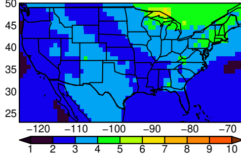
MRI-ESM2-0 tasmin JJA ssp370
