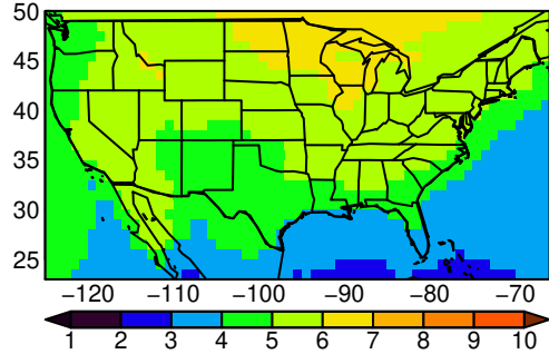
HadGEM3-GC31-LL tasmin yearly ssp2
