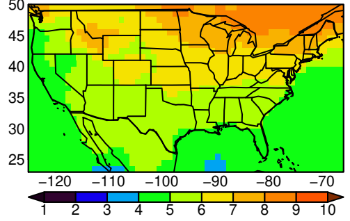
HadGEM3-GC31-LL tasmin JJA ssp5
