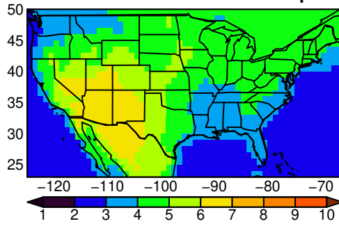
CNRM-CM6-1 tasmx JJA ssp370
