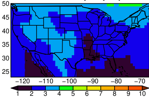
NESM3 tasmax yearly ssp245
