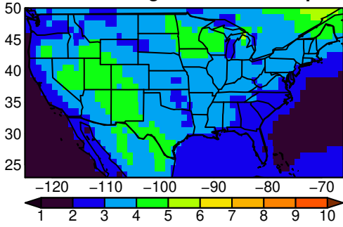
EC-Earth3-Veg tasmax JJA ssp245
