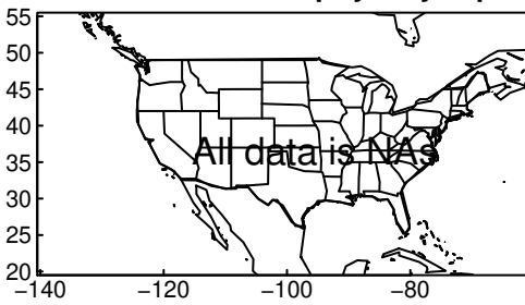
HadGEM3-GC31-LL pr yearly ssp370
