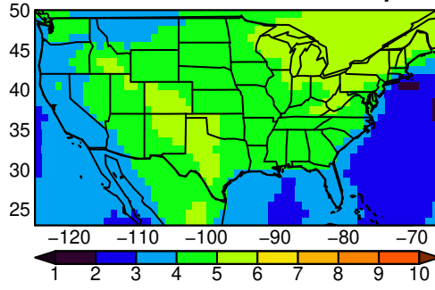
ACCESS-CM2 tasmax JJA ssp370
