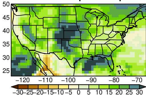
UKESM1-0-LL pr JJA ssp245
