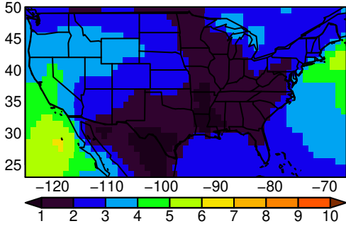
NESM3 tasmin yearly ssp245
