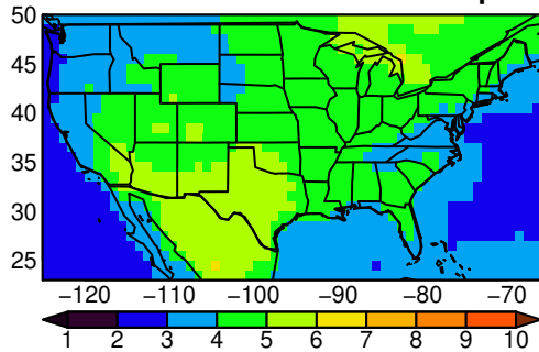
CNRM-ESM2-1 tasmin JJA ssp585
