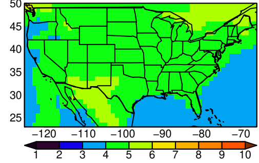
ACCESS-ESM1-5 tasmin JJA ssp58i
