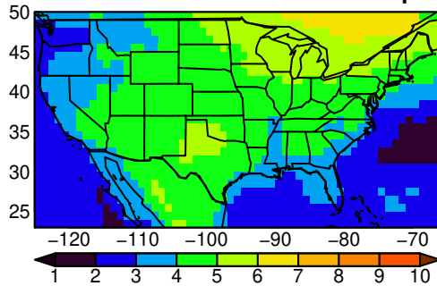
MPI-ESM1-2-HR tasmax JJA ssp58i
