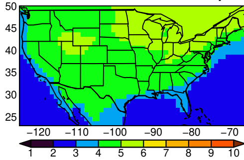
BCC-CSM2-MR tasmax yearly ssp370
