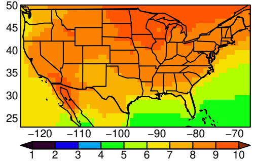
HadGEM3-GC31-LL tasmin yearly ssp5
