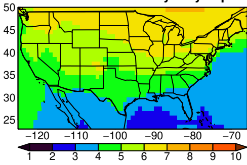
UKESM1-0-LL tasmax yearly ssp245
