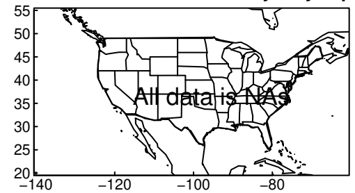
HadGEM3-GC31-MM tasmax yearly ssp5
