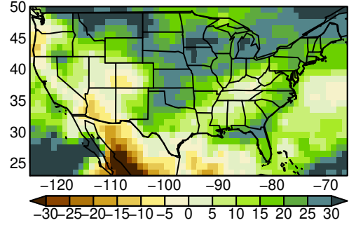
HadGEM3-GC31-LL pr JJA ssp585
