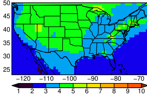
MRI-ESM2-0 tasmin SON ssp370
