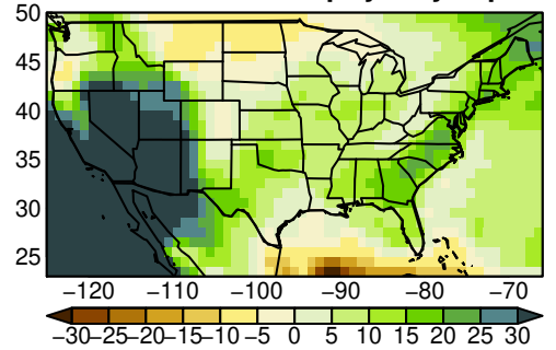
HadGEM3-GC31-LL pr yearly ssp585
