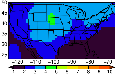
MPI-ESM1-2-LR tasmax yearly ssp24f
