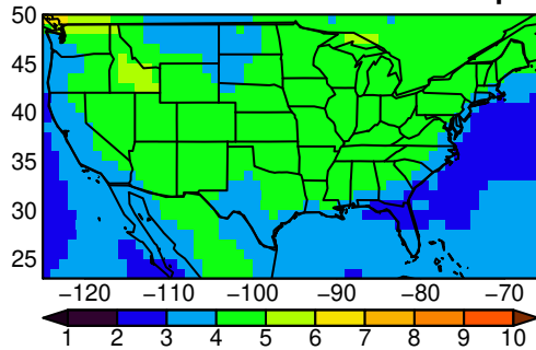
ACCESS-ESM1-5 tasmax JJA ssp37
