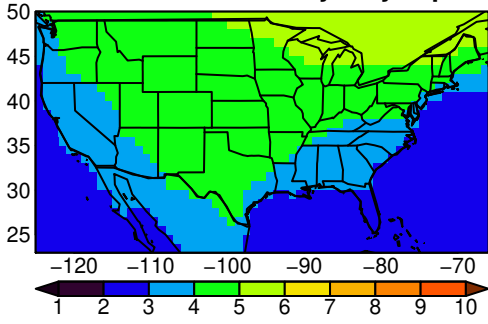
ACCESS-CM2 tasmax yearly ssp245
