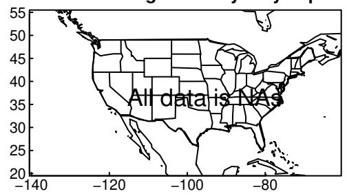
EC-Earth3-Veg tasmax yearly ssp585
