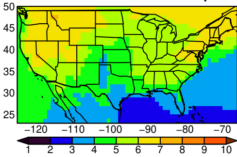
UKESM1-0-LL tasmin SON ssp245
