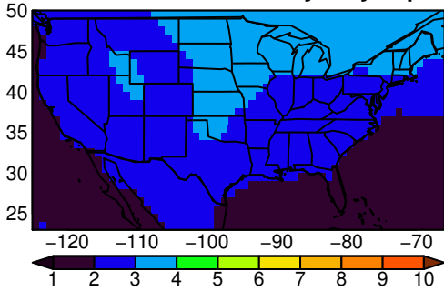
MPI-ESM1-2-LR tasmin yearly ssp245
