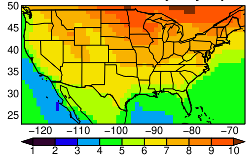
IPSL-CM6A-LR tasmin yearly ssp585
