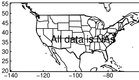
CESM2-FV2 pr yearly ssp370
