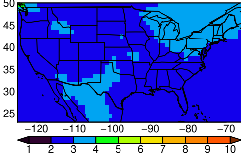
ACCESS-ESM1-5 tasmin JJA ssp24i
