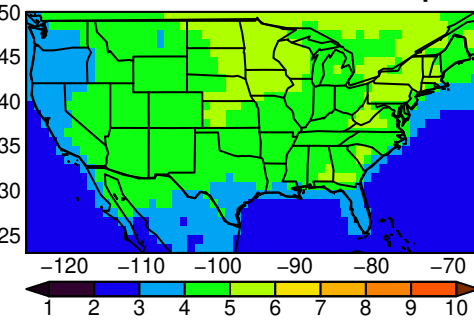
BCC-CSM2-MR tasmin yearly ssp370
