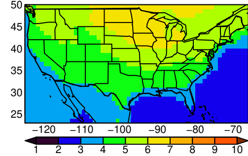
HadGEM3-GC31-LL tasmax yearly ssp2
