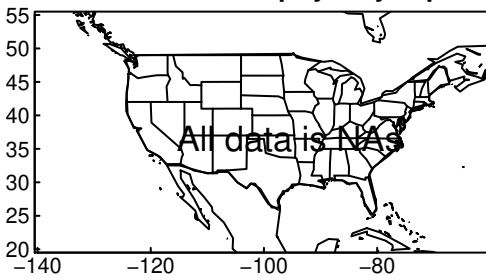
CNRM-CM6-1-HR pr yearly ssp245
