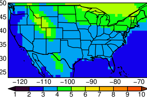
BCC-CSM2-MR tasmin JJA ssp370
