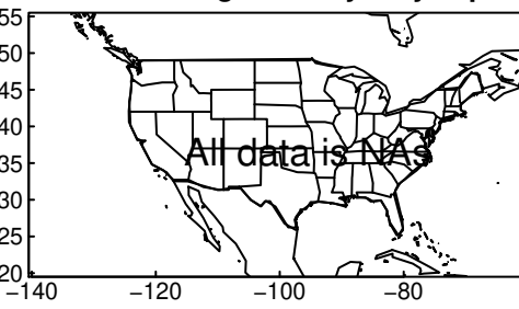
EC-Earth3-Veg tasmin yearly ssp370
