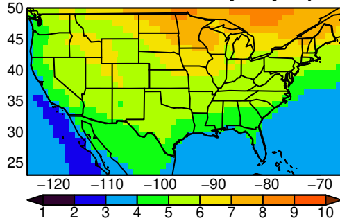
IPSL-CM6A-LR tasmin yearly ssp370
