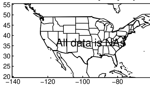
GISS-E2-1-G tasmin yearly ssp370
