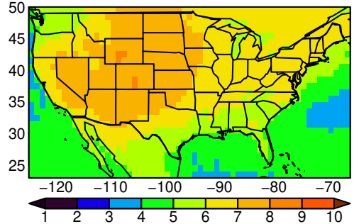
CNRM-CM6-1-HR tasmax yearly ssp5
