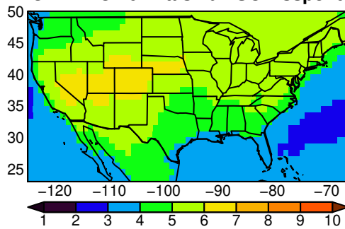
CNRM-CM6-1 tasmx yearly ssp370
