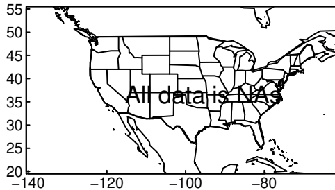
EC-Earth3-Veg pr yearly ssp585
