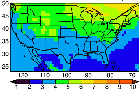
UKESM1-0-LL tasmin JJA ssp245
