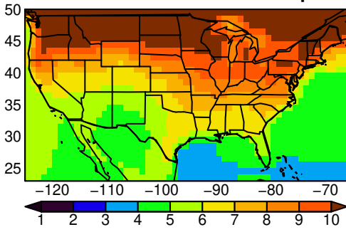
UKESM1-0-LL tasmax SON ssp370
