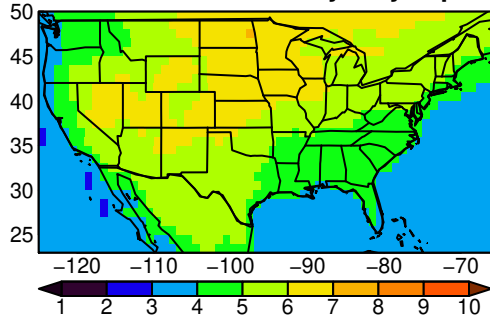
CNRM-ESM2-1 tasmin yearly ssp585
