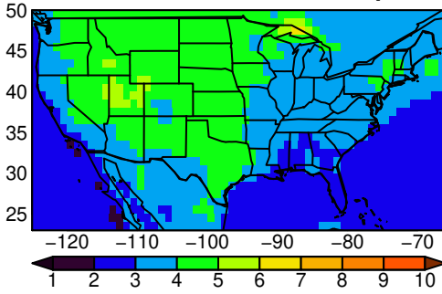
MRI-ESM2-0 tasmax SON ssp370
