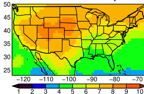
NESM3 tasmax yearly ssp585
