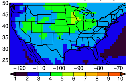
CNRM-ESM2-1 tasmin yearly ssp245
