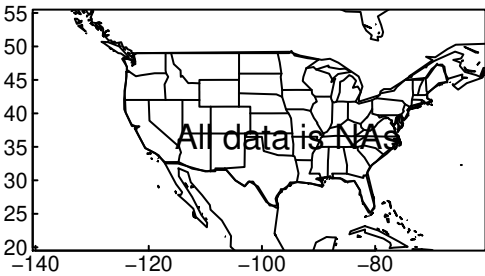
CNRM-CM6-1-HR tasmax yearly ssp2
