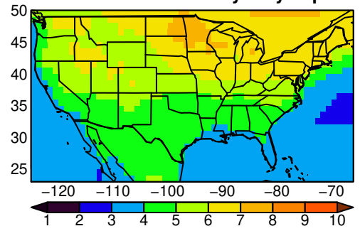
NorESM2-MM tasmx yearly ssp585
