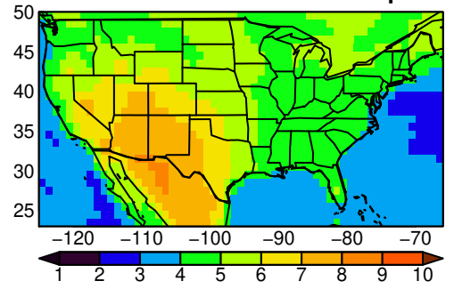
CNRM-CM6-1 tasmx JJA ssp585
