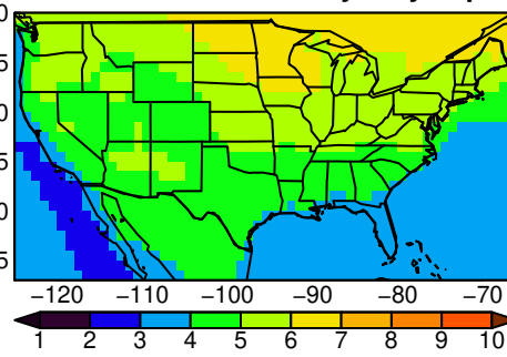
IPSL-CM6A-LR tasmax yearly ssp370
