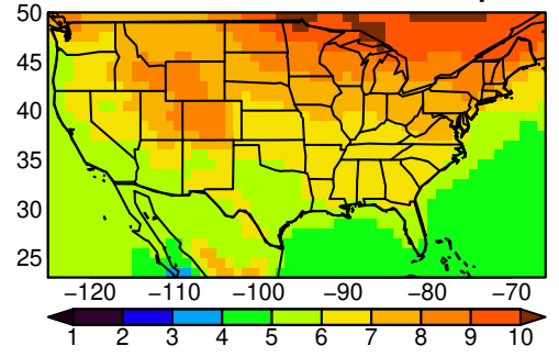
UKESM1-0-LL tasmin JJA ssp585
