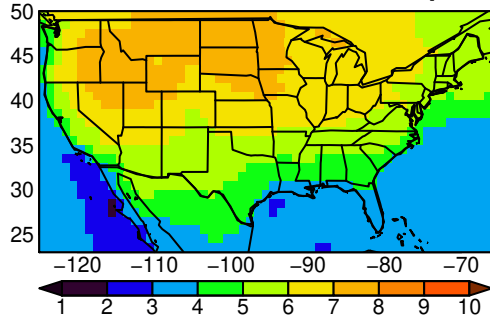
IPSL-CM6A-LR tasmin SON ssp370
