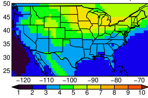
NorESM2-MM tasmx JJA ssp370
