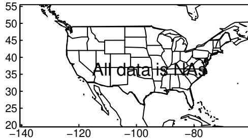
HadGEM3-GC31-LL tasmin JJA ssp3
