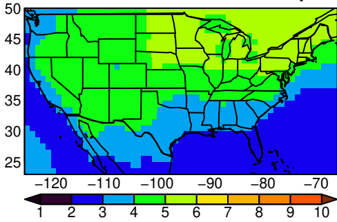
IPSL-CM6A-LR tasmax yearly ssp245
