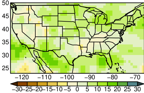
FGOALS-g3 pr yearly ssp245
