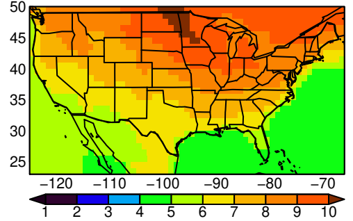
HadGEM3-GC31-LL tasmax yearly ssp5
