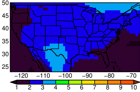
MPI-ESM1-2-LR tasmax JJA ssp24f
