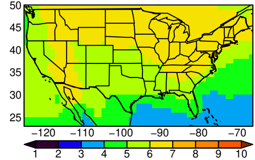
ACCESS-ESM1-5 tasmin yearly ssp58i
