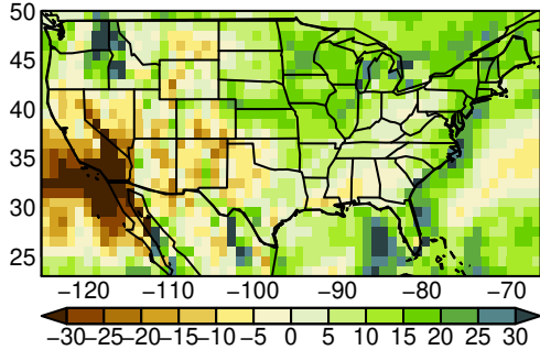
EC-Earth3-Veg pr yearly ssp245
