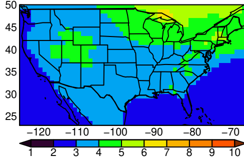
MRI-ESM2-0 tasmin yearly ssp370
