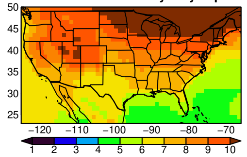
UKESM1-0-LL tasmin yearly ssp585
