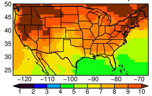
UKESM1-0-LL tasmin SON ssp585
