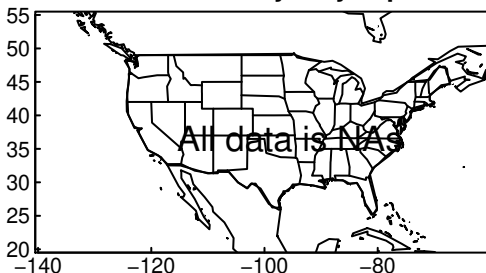
NESM3 tasmax yearly ssp370
