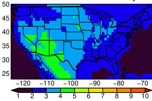
CNRM-CM6-1 tasmx JJA ssp245
