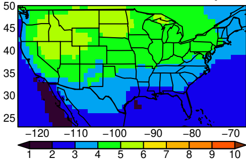
IPSL-CM6A-LR tasmin SON ssp245
