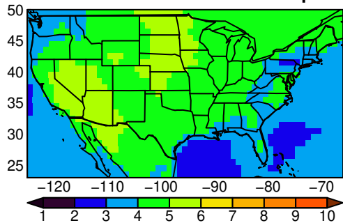
CNRM-ESM2-1 tasmin yearly ssp370
