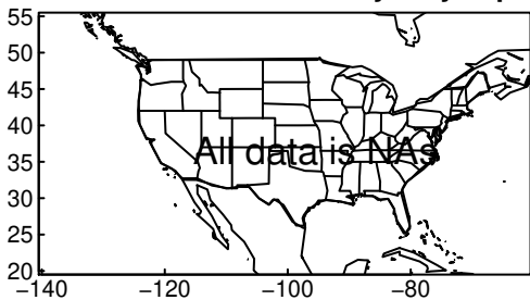
CNRM-CM6-1-HR tasmin yearly ssp2
