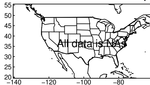
HadGEM3-GC31-MM tasmin JJA ssp5
