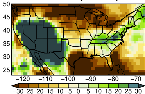
UKESM1-0-LL pr SON ssp370
