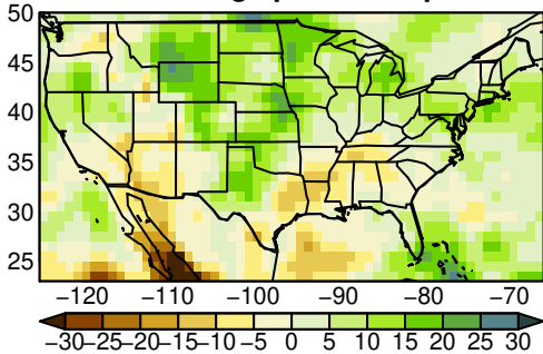
FGOALS-g3 pr JJA ssp245
