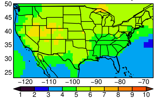
MRI-ESM2-0 tasmax yearly ssp585
