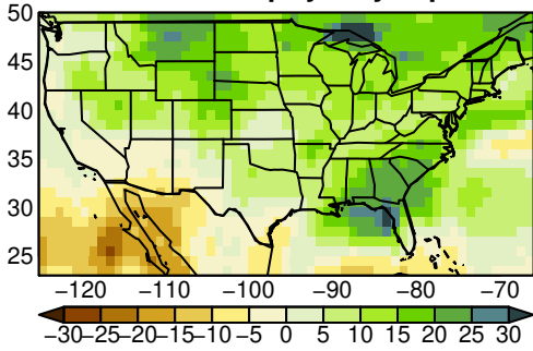
MRI-ESM2-0 pr yearly ssp245
