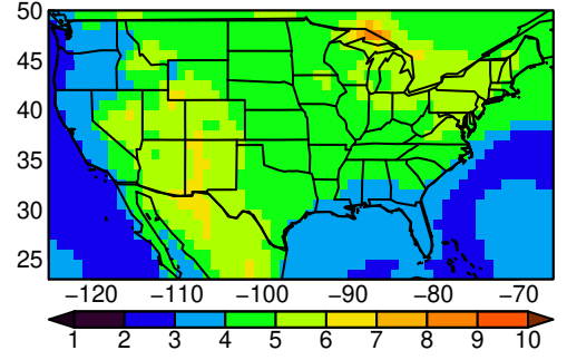
MRI-ESM2-0 tasmax JJA ssp585
