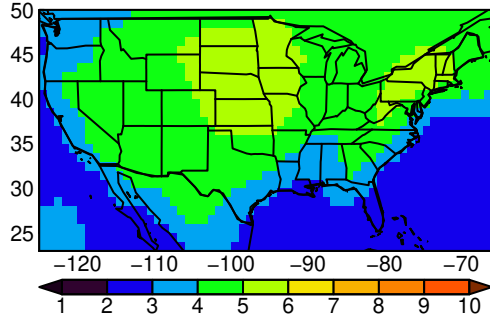
MPI-ESM1-2-LR tasmax yearly ssp37f
