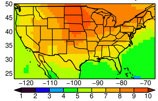
ACCESS-CM2 tasmax yearly ssp585
