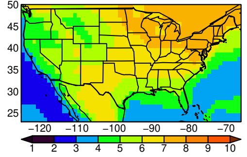
IPSL-CM6A-LR tasmax JJA ssp585
