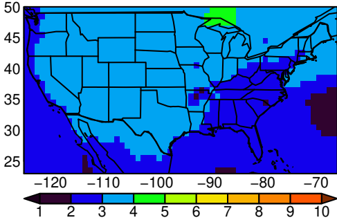
MRI-ESM2-0 tasmin yearly ssp245
