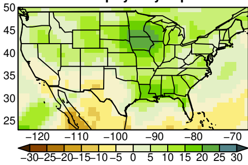
NESM3 pr yearly ssp245
