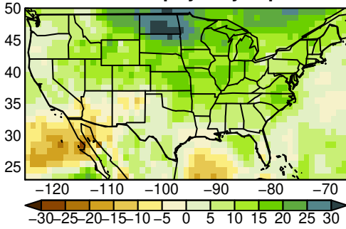
EC-Earth3 pr yearly ssp370
