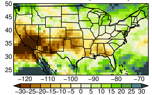
CNRM-CM6-1-HR pr yearly ssp585
