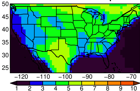
NESM3 tasmax JJA ssp245
