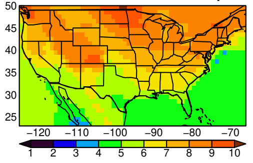
UKESM1-0-LL tasmax JJA ssp585
