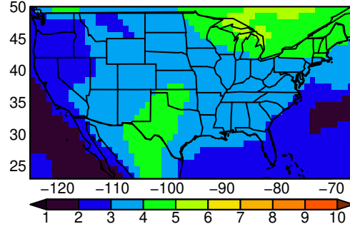
MPI-ESM1-2-LR tasmin JJA ssp370
