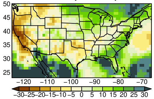
EC-Earth3 pr yearly ssp585
