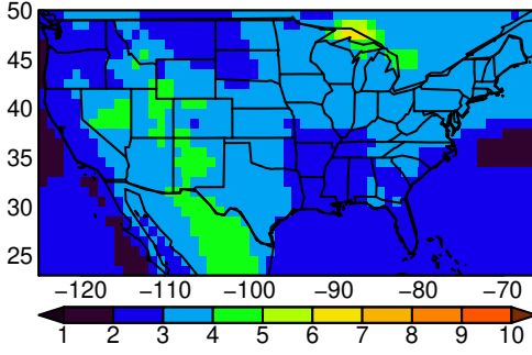
MRI-ESM2-0 tasmax JJA ssp370
