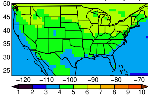
ACCESS-ESM1-5 tasmax yearly ssp37
