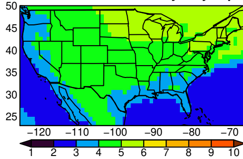
AWI-CM-1-1-MR tasmax yearly ssp37i
