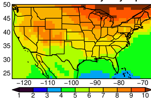
UKESM1-0-LL tasmin yearly ssp370
