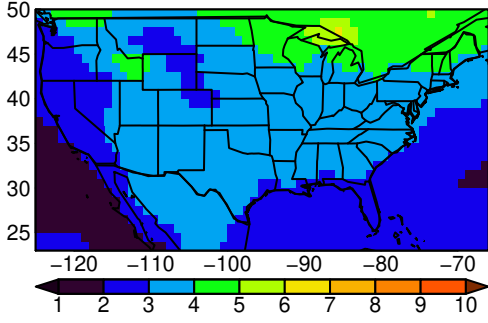
IPSL-CM6A-LR tasmin JJA ssp245
