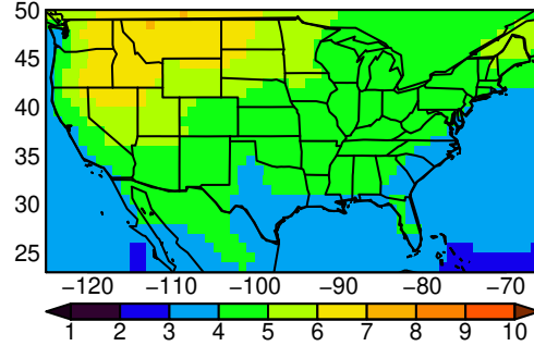
ACCESS-ESM1-5 tasmin SON ssp37i
