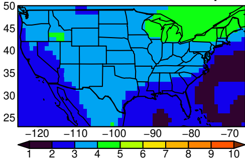
ACCESS-CM2 tasmax JJA ssp245
