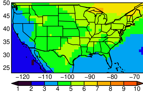
IPSL-CM6A-LR tasmin JJA ssp370
