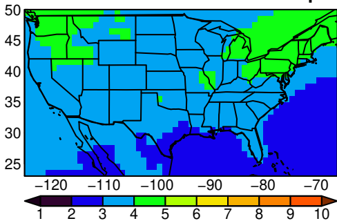
ACCESS-ESM1-5 tasmax yearly ssp24
