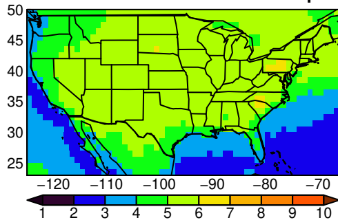
AWI-CM-1-1-MR tasmin yearly ssp37f
