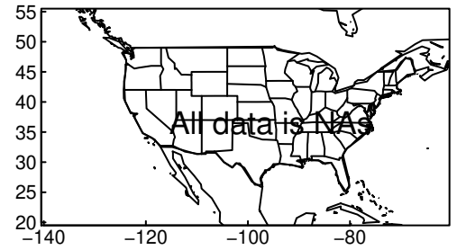
MPI-ESM1-2-LR tasmax yearly ssp58f
