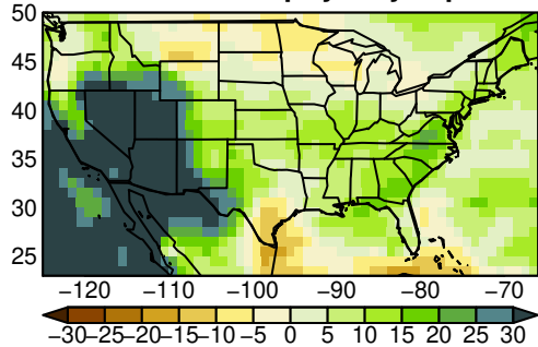
UKESM1-0-LL pr yearly ssp370
