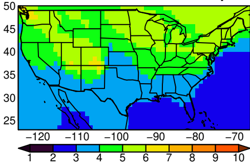
UKESM1-0-LL tasmax JJA ssp245
