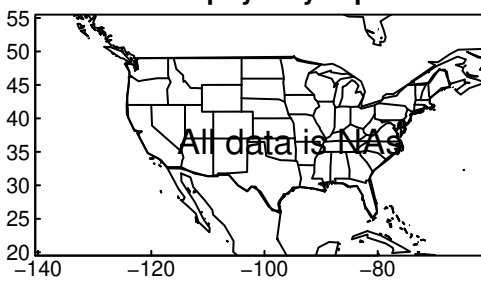
NESM3 pr yearly ssp370
