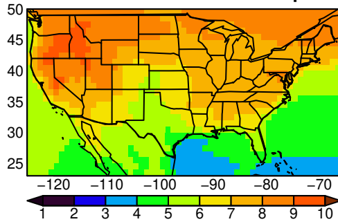
UKESM1-0-LL tasmin SON ssp370
