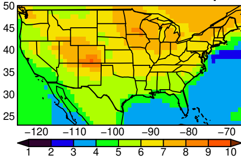
UKESM1-0-LL tasmax JJA ssp370
