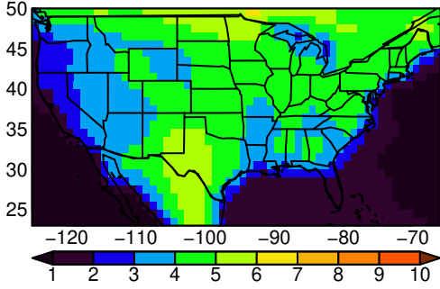
NESM3 tasmin JJA ssp245
