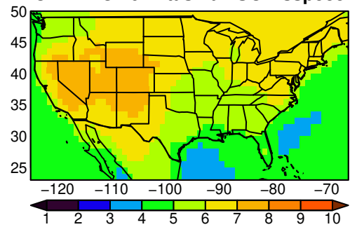
CNRM-CM6-1 tasmx yearly ssp585
