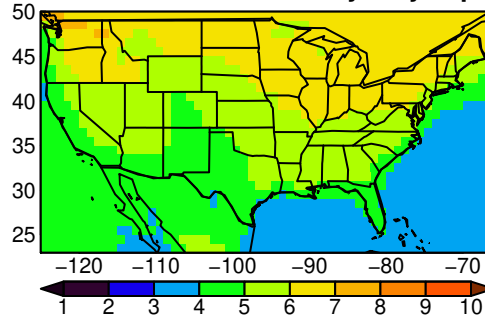
ACCESS-ESM1-5 tasmax yearly ssp58
