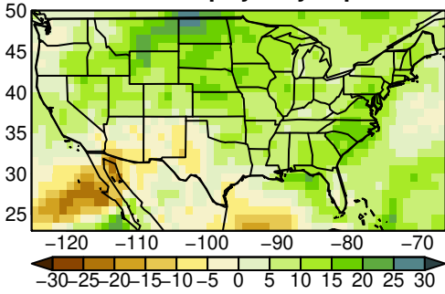
EC-Earth3 pr yearly ssp245
