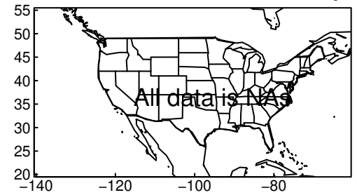
HadGEM3-GC31-MM tasmax JJA ssp5
