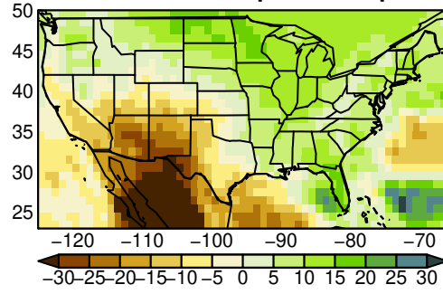
MPI-ESM1-2-HR pr JJA ssp370
