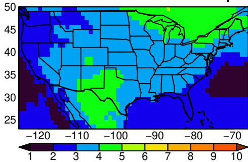
MPI-ESM1-2-HR tasmax JJA ssp37i
