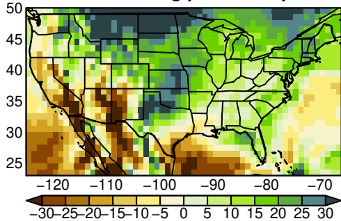
EC-Earth3-Veg pr JJA ssp245
