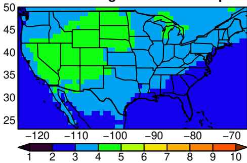
EC-Earth3-Veg tasmax yearly ssp245
