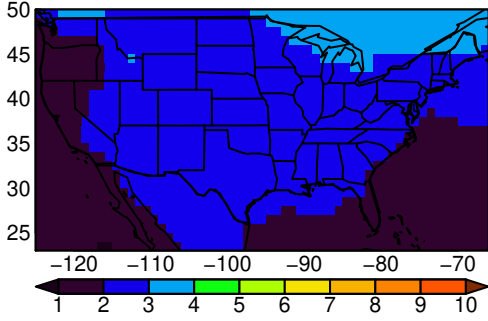
MPI-ESM1-2-LR tasmin JJA ssp245
