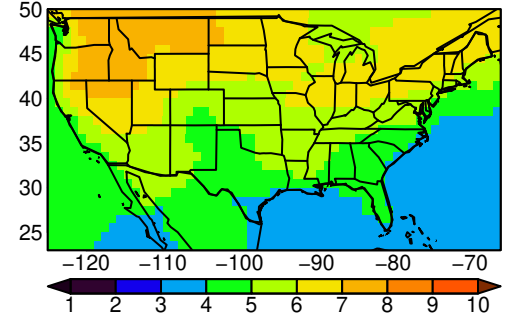
ACCESS-ESM1-5 tasmin SON ssp58i
