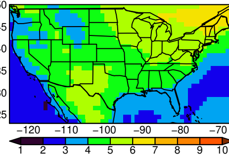
IPSL-CM6A-LR tasmax JJA ssp370
