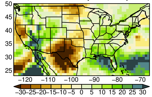
MPI-ESM1-2-HR pr yearly ssp585
