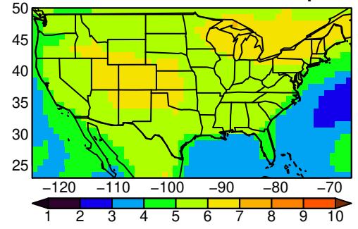
ACCESS-CM2 tasmax JJA ssp585
