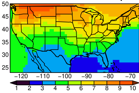
UKESM1-0-LL tasmax SON ssp245
