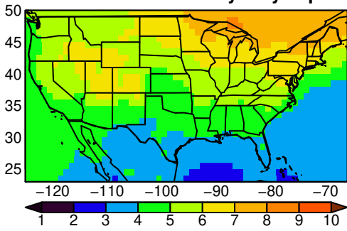
UKESM1-0-LL tasmin yearly ssp245
