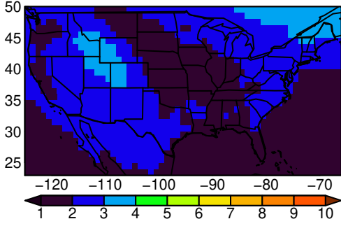
BCC-CSM2-MR tasmin JJA ssp245
