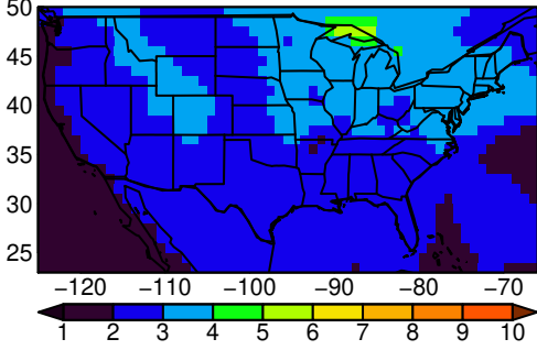
MRI-ESM2-0 tasmin JJA ssp245
