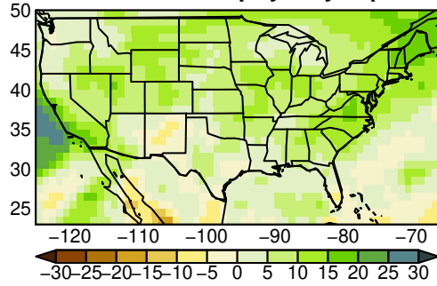
BCC-CSM2-MR pr yearly ssp370
