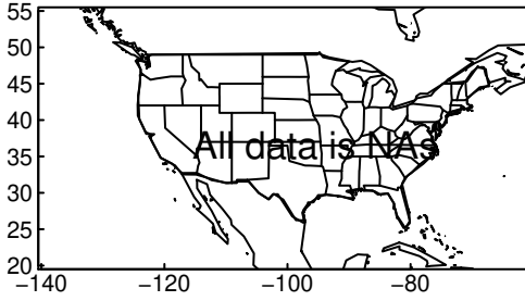
NESM3 tasmin DJF ssp370
