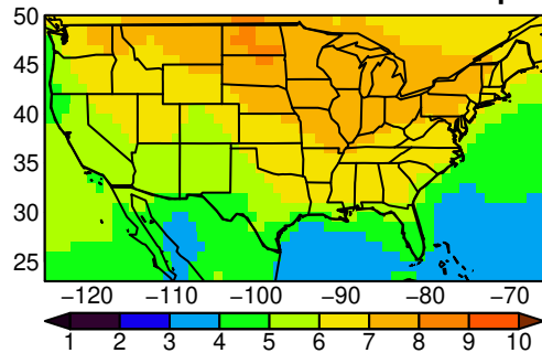
ACCESS-ESM1-5 tasmax yearly ssp58
