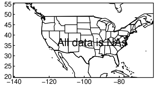
TaiESM1 tasmin yearly ssp585
