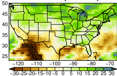
IPSL-CM6A-LR pr JJA ssp245
