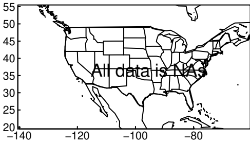
TaiESM1 tasmin yearly ssp245
