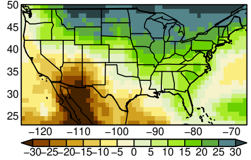
MMEA-MEDIAN pr JJA ssp585 n= 16
