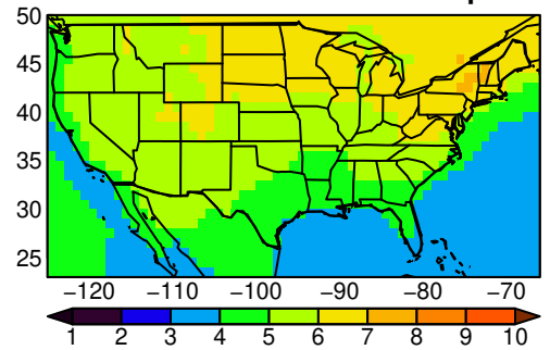
NorESM2-MM tasmax yearly ssp585
