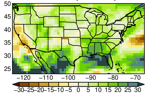
MRI-ESM2-0 pr yearly ssp585
