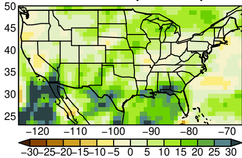
BCC-CSM2-MR pr yearly ssp245
