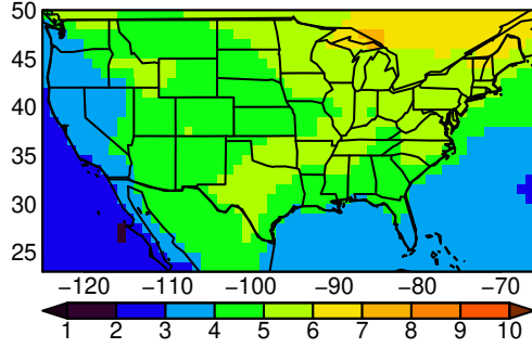
IPSL-CM6A-LR tasmin JJA ssp370
