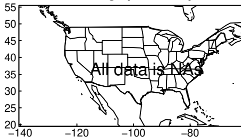
FGOALS-g3 pr DJF ssp585
