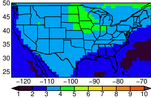
MMEA-MEDIAN tasmx yearly ssp245 n=
