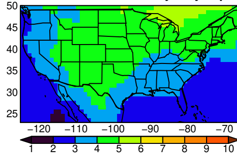
MPI-ESM1-2-LR tasmin yearly ssp370
