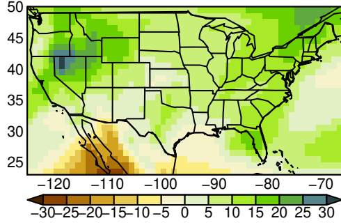
CESM2 pr yearly ssp370
