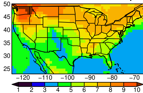
ACCESS-ESM1-5 tasmax SON ssp58
