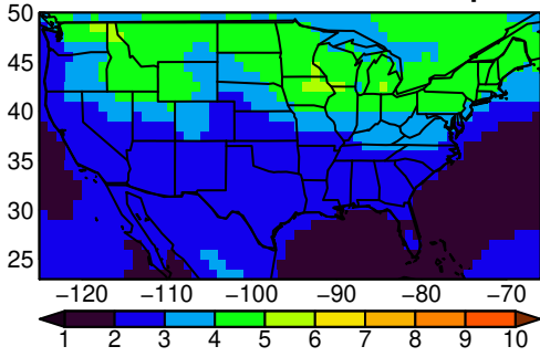
NorESM2-MM tasmax JJA ssp245
