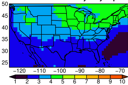
NorESM2-MM tasmax yearly ssp245
