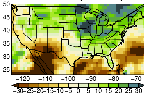
IPSL-CM6A-LR pr JJA ssp585
