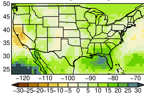
MMEA-MEDIAN pr yearly ssp370 n= 1
