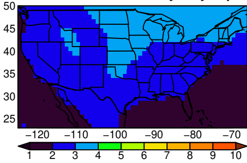
MPI-ESM1-2-LR tasmin yearly ssp245
