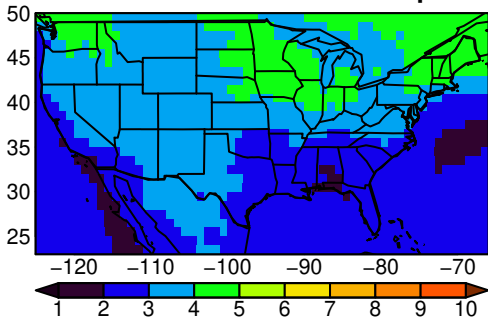
NorESM2-MM tasmax SON ssp245
