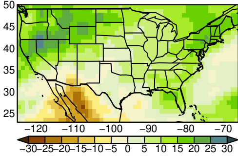
CESM2 pr yearly ssp245
