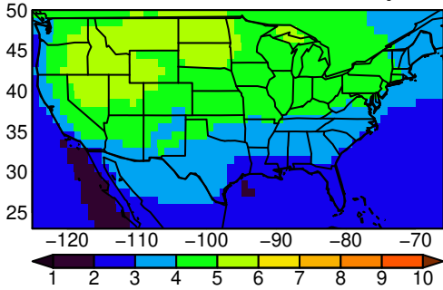
IPSL-CM6A-LR tasmin SON ssp245
