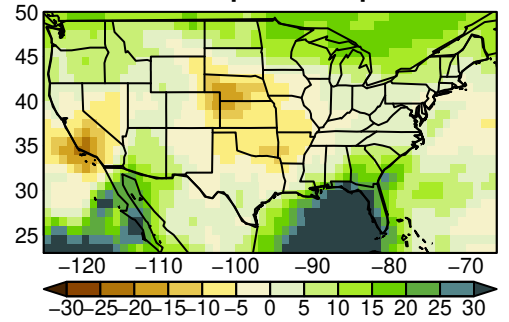
MIROC6 pr yearly ssp585
