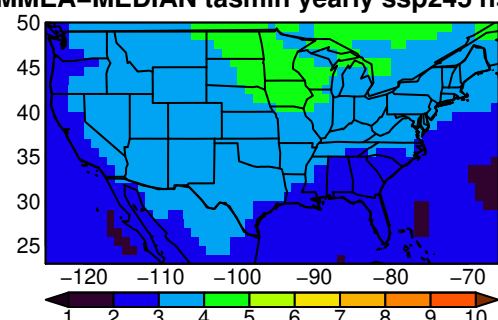
MMEA-MEDIAN tasmin yearly ssp245 n=
