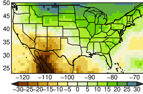
MMEA-MEDIAN pr JJA ssp370 n= 17
