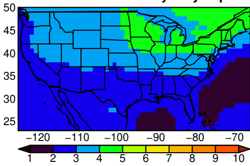
NorESM2-LM tasmx yearly ssp245
