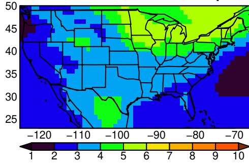
NorESM2-LM tasmx JJA ssp370
