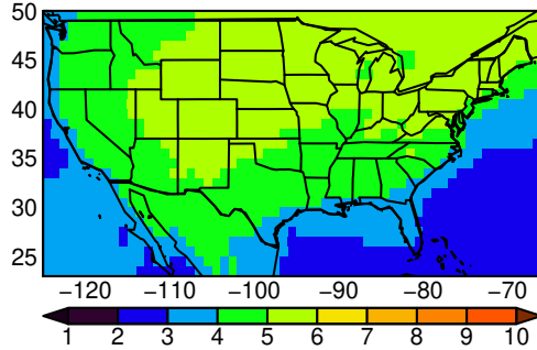
MMEA-MEDIAN tasmx yearly ssp370 n=
