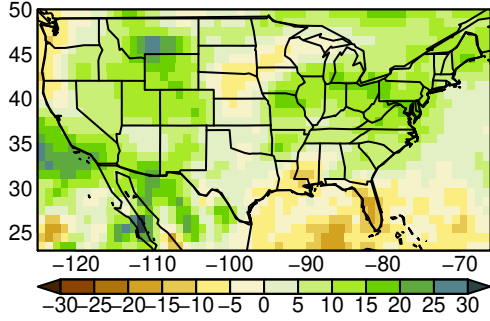
BCC-CSM2-MR pr JJA ssp245
