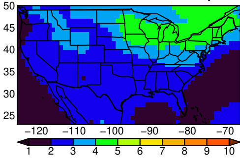
NorESM2-LM tasmx JJA ssp245
