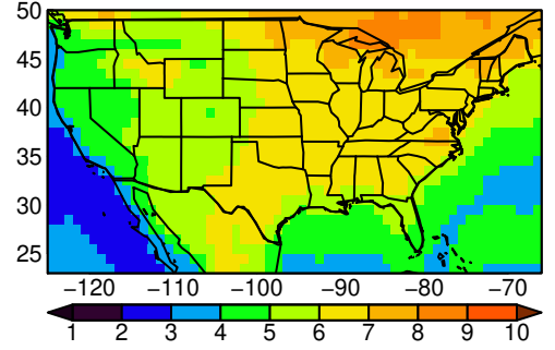
IPSL-CM6A-LR tasmin JJA ssp585
