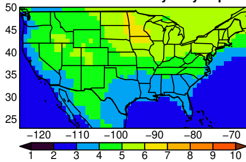
NorESM2-MM tasmax yearly ssp370
