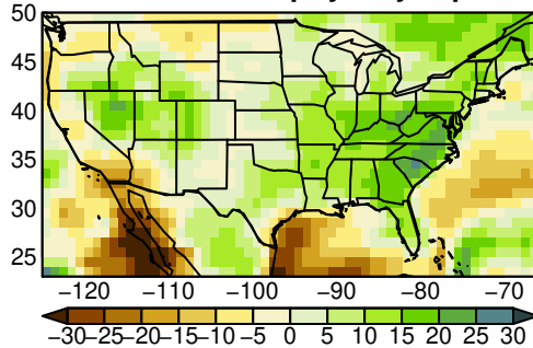
IPSL-CM6A-LR pr yearly ssp585
