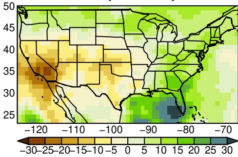
MIROC6 pr yearly ssp245
