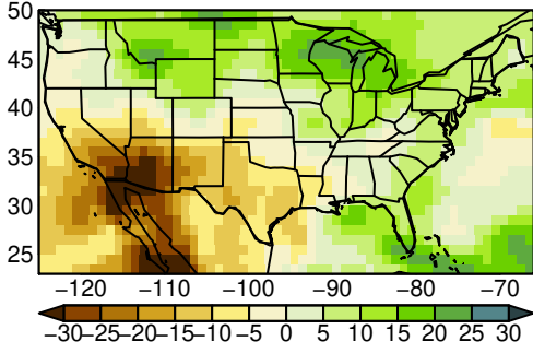
MIROC6 pr JJA ssp245
