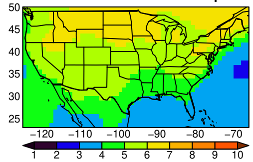
NorESM2-LM tasmx yearly ssp585
