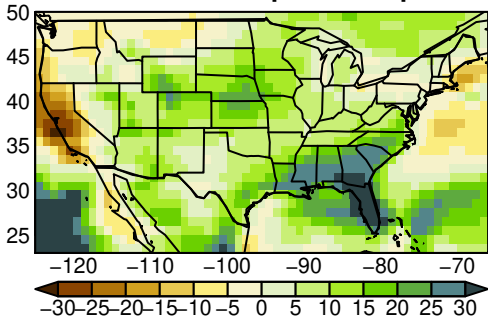
IPSL-CM6A-LR pr yearly ssp370
