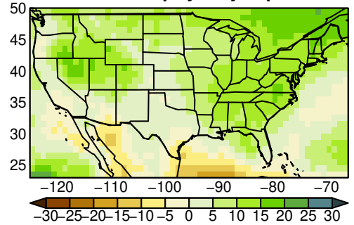
MMEA-MEDIAN pr yearly ssp585 n= 1
