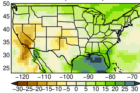
MIROC6 pr yearly ssp370
