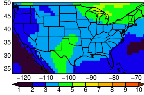
MPI-ESM1-2-LR tasmin JJA ssp370
