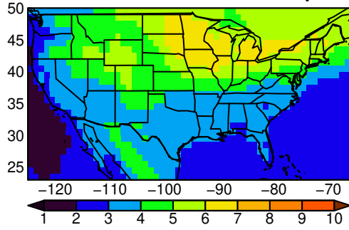
NorESM2-MM tasmax JJA ssp370
