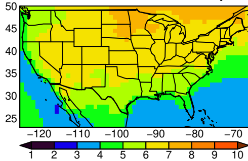
IPSL-CM6A-LR tasmin yearly ssp370
