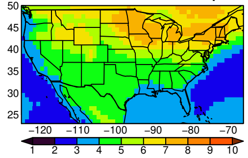
NorESM2-MM tasmax JJA ssp585
