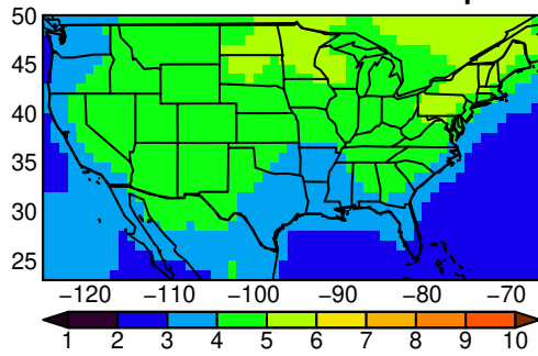
NorESM2-LM tasmx yearly ssp370
