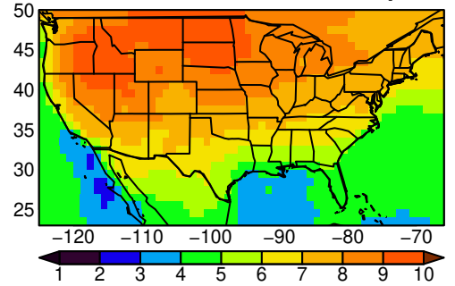
IPSL-CM6A-LR tasmin SON ssp585
