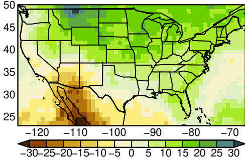
MMEA-MEDIAN pr JJA ssp245 n= 21
