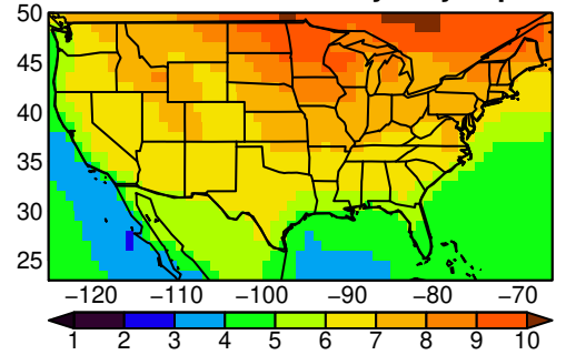
IPSL-CM6A-LR tasmin yearly ssp585
