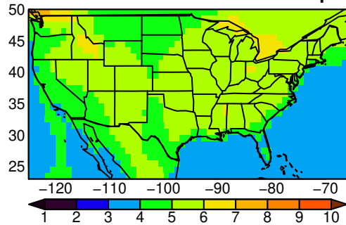
ACCESS-ESM1-5 tasmax JJA ssp58
