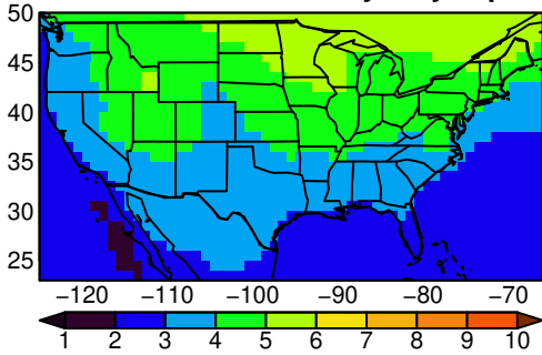
IPSL-CM6A-LR tasmin yearly ssp245
