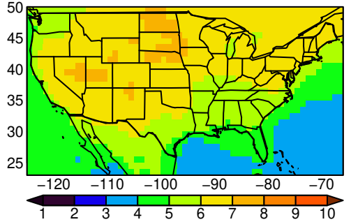
MMEA-MEDIAN tasmx yearly ssp585 n=
