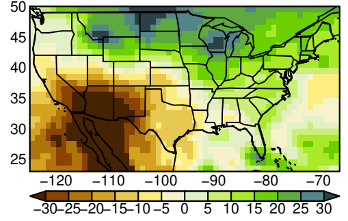
MIROC6 pr JJA ssp585
