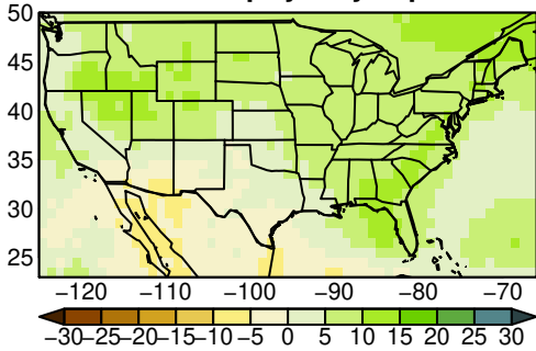
MMEA-MEDIAN pr yearly ssp245 n= 2
