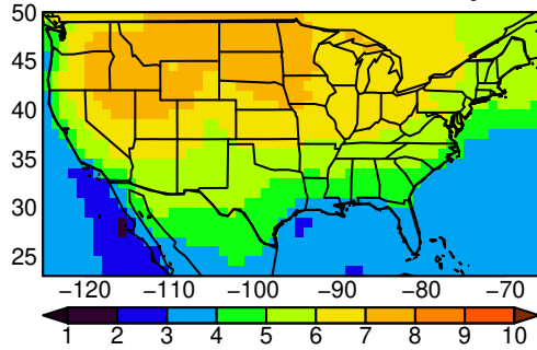
IPSL-CM6A-LR tasmin SON ssp370
