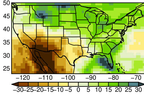
MIROC6 pr JJA ssp370
