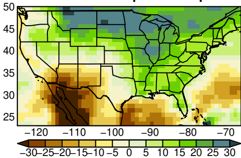
IPSL-CM6A-LR pr JJA ssp370
