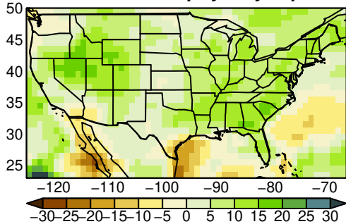
IPSL-CM6A-LR pr yearly ssp245
